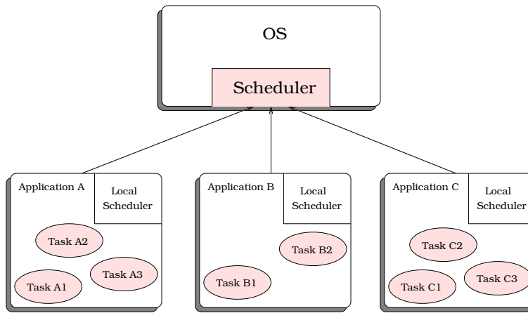
Fig. 1. A hierarchical scheduler.
