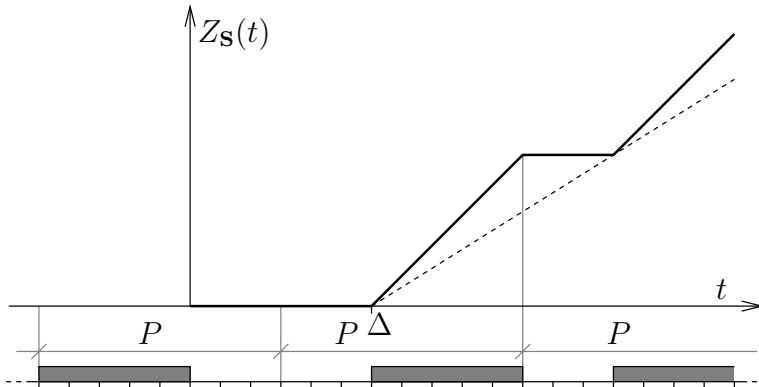
Fig. 3. Characteristic function of server S = (5, 8) .
