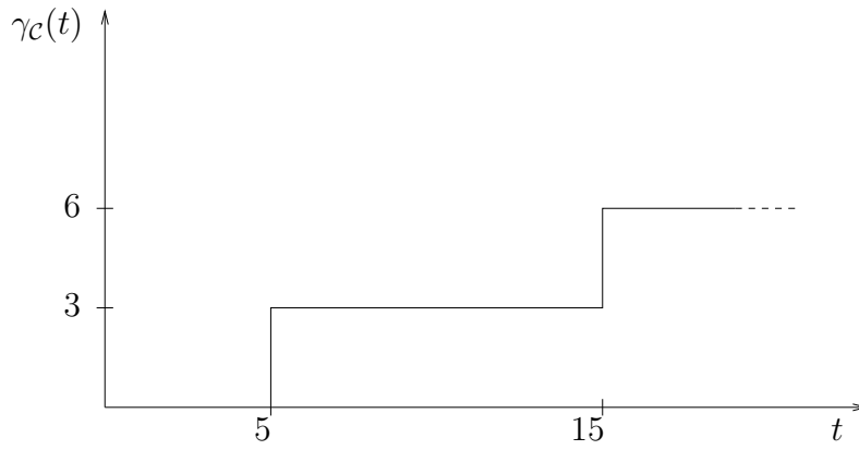
Fig. 2. Function \gamma_{\mathcal{C}}(t) for the component in the example.
